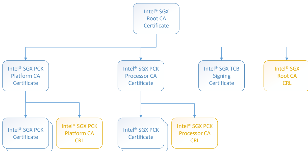
Figure 0-1: Certificate Hierarchy
